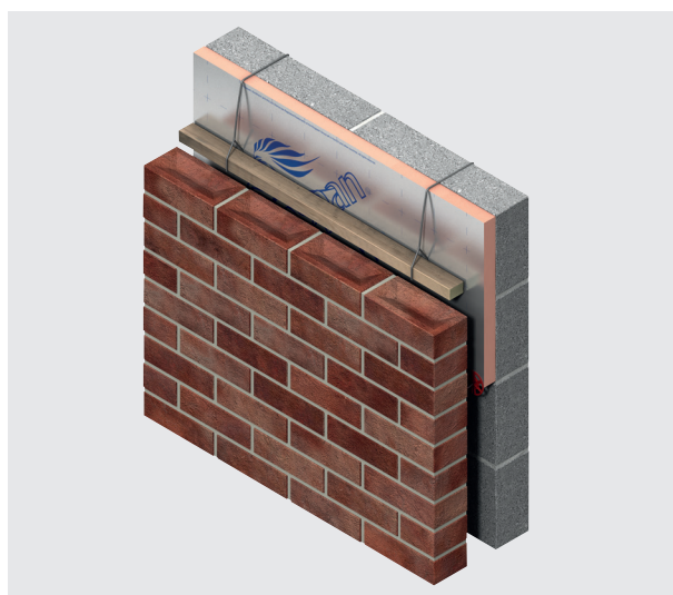
Figure 8: Use of a cavity batten to protect the cavity
